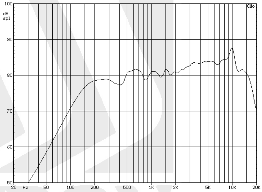
Typical Frequency Response
