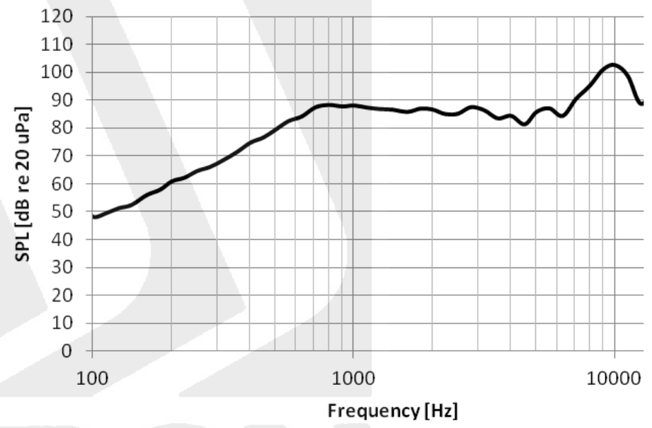
Typical Frequency Response
