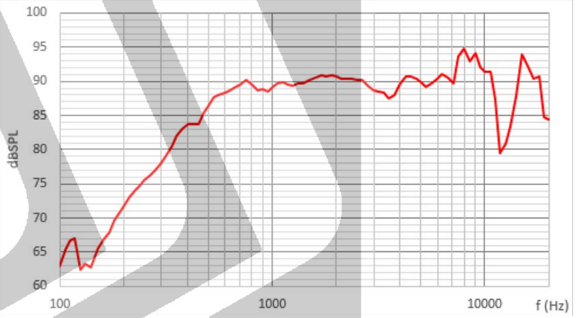
Typical Frequency Response
