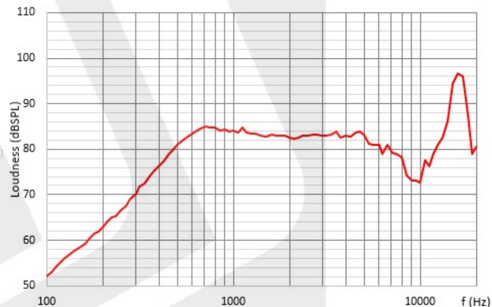
Typical Frequency Response
